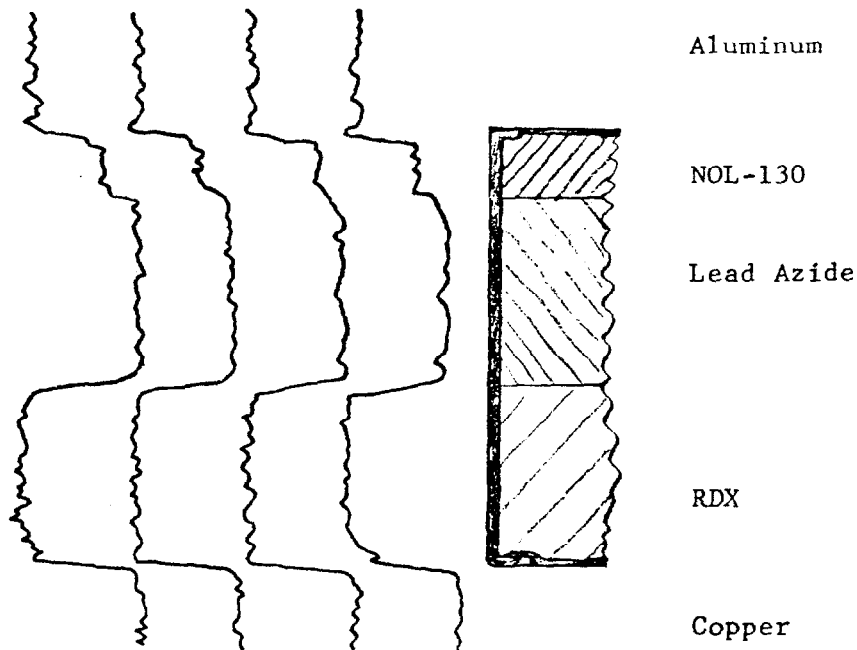
Fig 7 Typical \gamma -Ray Densitometer Scan of an M-55 Detonator
